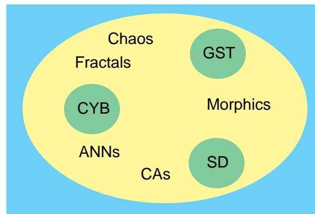
Figure 7. The branches of complexity. Here we show just a few of the more active math branches.
