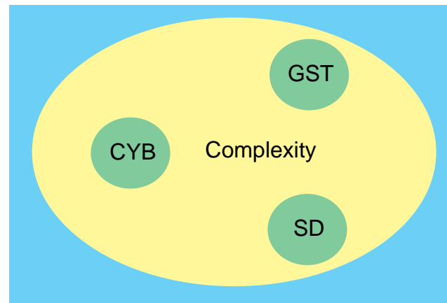
Figure 6. The trunk of complexity. Here, the central (link) zone is widened.
